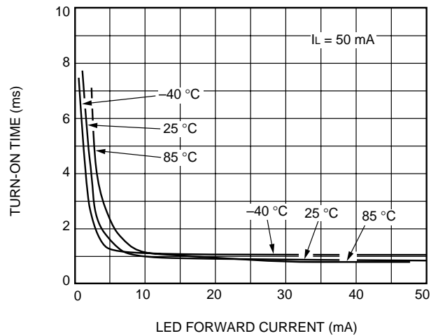
B. Turn-On Time vs. LED Current (LH1522)
